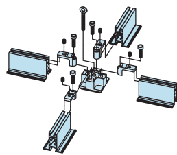
Type CK
