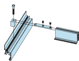
Type WC 1
